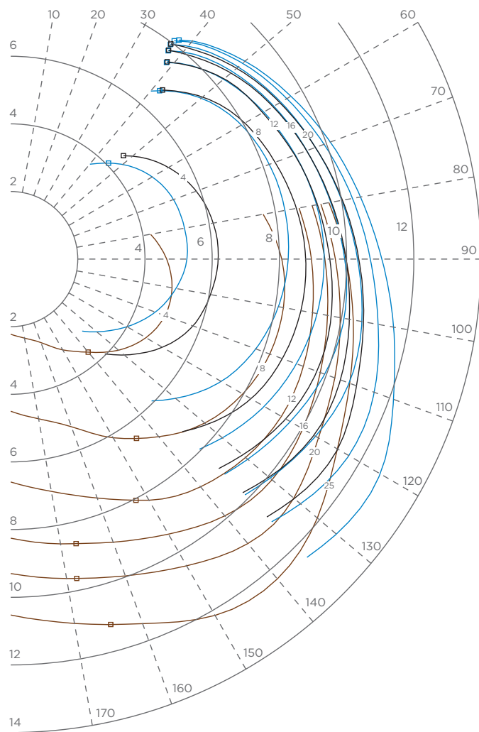
POLAR DIAGRAM Performance keel, performance mast and membrane sails
